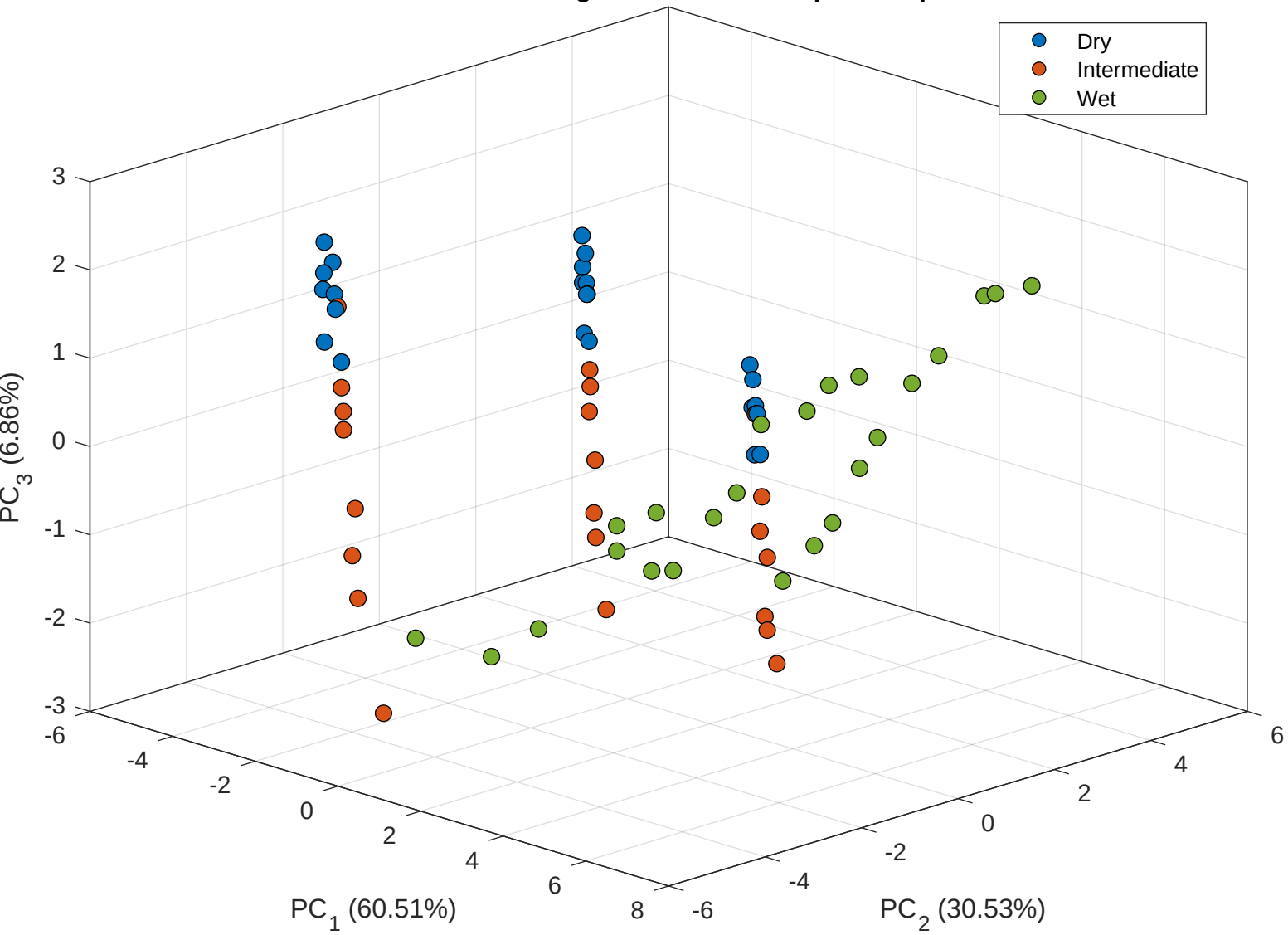
PCA Score Plot Using Selected 3 Principal Components
